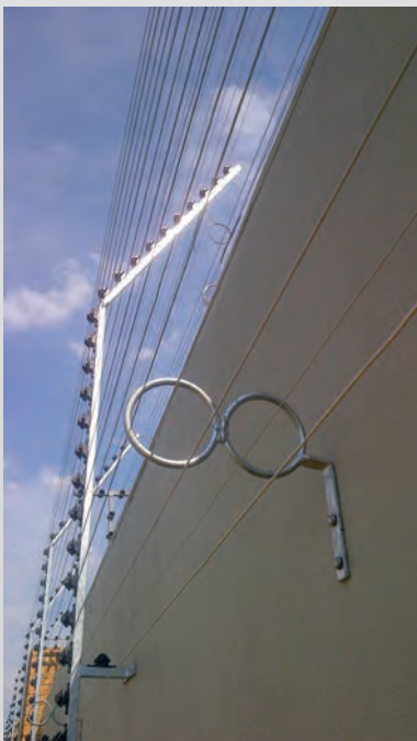
Bi-Polar Security SIS Series Monitor Loop Allows for earth and live monitoring or Bi-Polar monitoring
